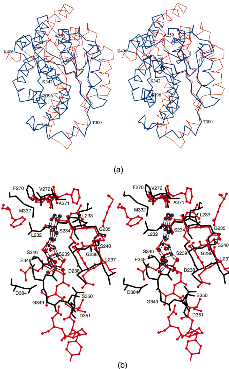
FIGURE 6: Comparison of the acceptor domains in asparagine synthetase and GMP synthetase. X-ray coordinates for GMP synthetase (9) were obtained from the Brookhaven Protein Data Bank (1GPM). A superposition of the \alpha -carbons for the C-terminal domains in asparagine synthetase (blue) and GMP synthetase (red) is depicted in panel a. A close-up view of the protein environment surrounding the nucleotides is displayed in panel b. For the sake of clarity, the Mg^{2+} ions and the pyrophosphate moiety in GMP synthetase and the uranium ions in asparagine synthetase were omitted.
